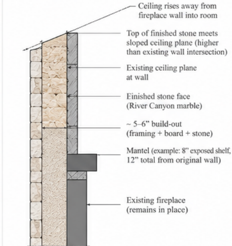
SIDE SECTION — PROJECTION & CEILING SLOPE
